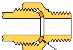
Copper Gasket
